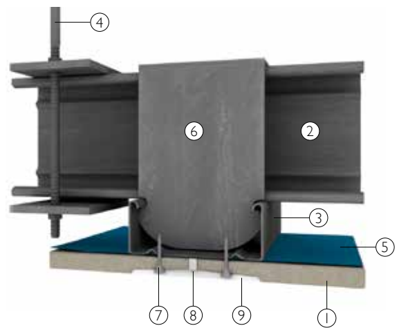
Joint detail
