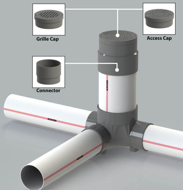
Connector 6" Access Cap 6"
